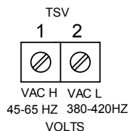
FIG. LPE-8/Y OPTIONS 8/Y VAC OR HZ SIGNAL POWERED
