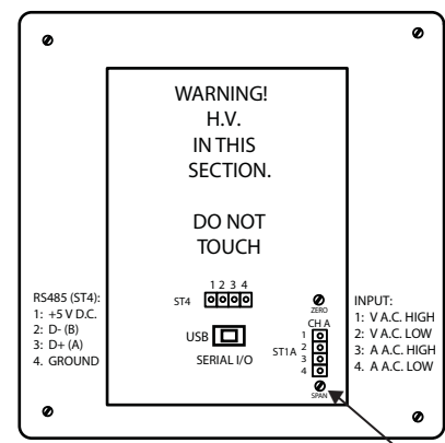
NTM-M & -N TYPICAL CONNECTIONS SIGNAL POWER MODELS
