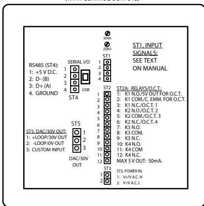
NTM-M & N TYPICAL CONNECTIONS EXTERNALLY POWERED MODELS (WITH CONTROL OUTPUTS)
