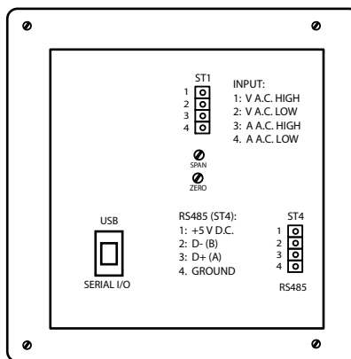
NTM-M & -N TYPICAL CONNECTIONS LOOP POWER/5 V.P./USB POWERED MODELS
