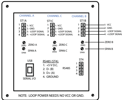
LOOP POWER OR 5 V.P./USB POWERED MODELS (NO CONTROL OUT)
