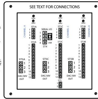
NTM-A TYPICAL CONNECTIONS EXTERNALLY POWERED MODELS (WITH CONTROL OUTPUTS)
