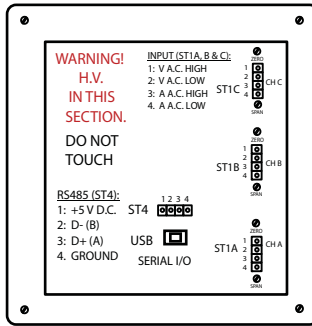
NTM-A TYPICAL CONNECTIONS SIGNAL POWERED MODELS
